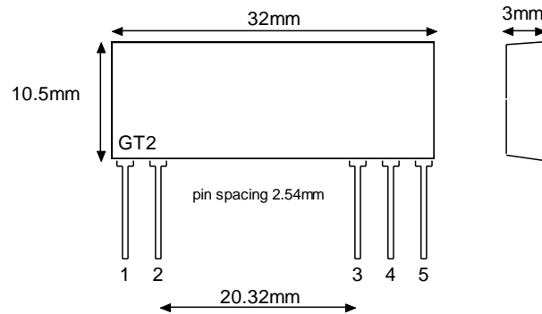
Figure 4: GT2 Transmitter
