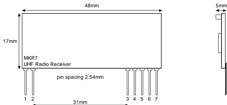
Figure 4: MKR7 Receiver
